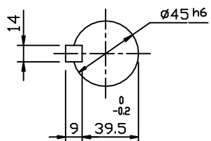
OUTPUT SHAFT
