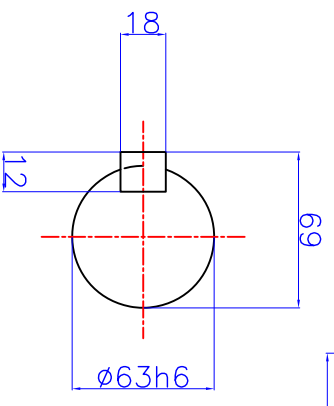
OUTPUT SHAFT
